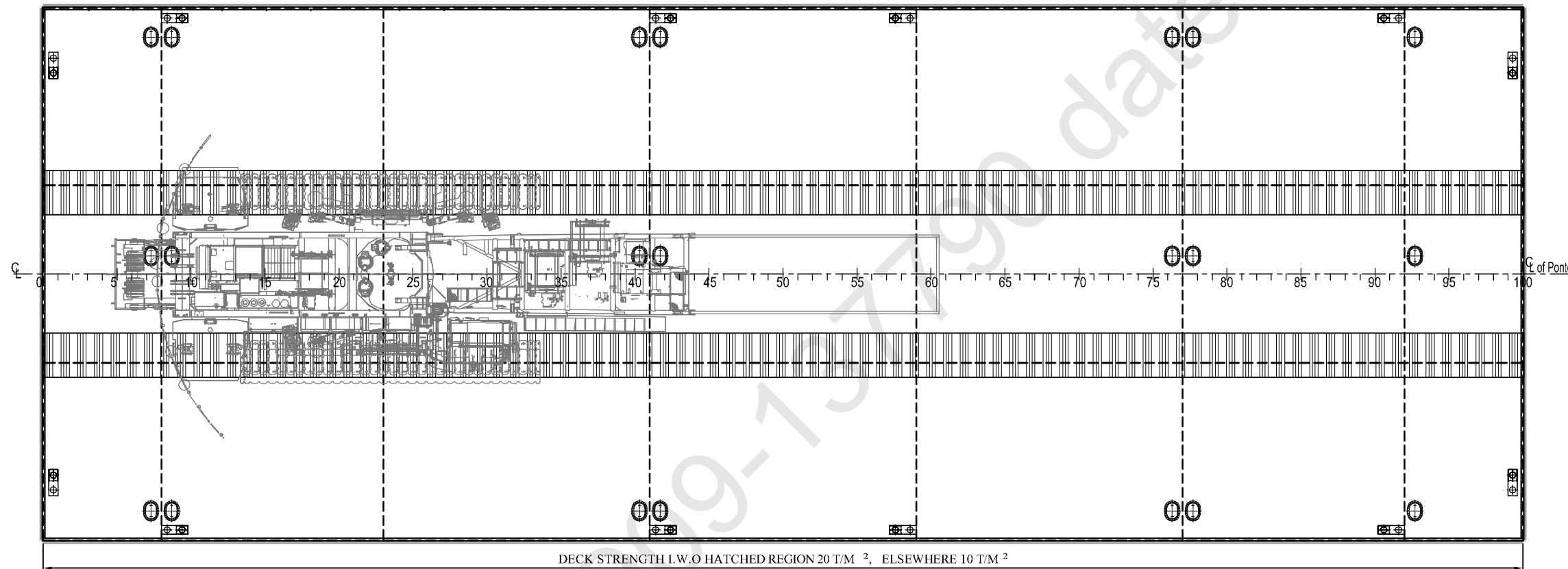
MAIN DECK PLAN
